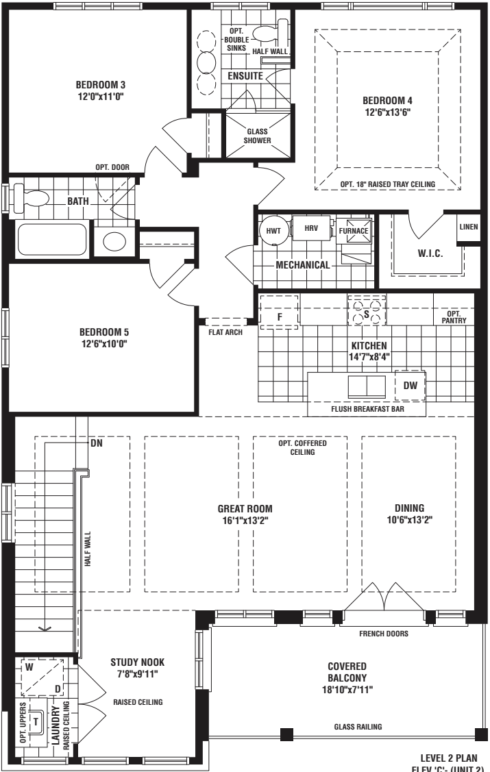
LEVEL 2 PLAN ELEV. 'C' - (UNIT 2)
